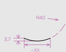
LAMEL KRAFT 6 detail
