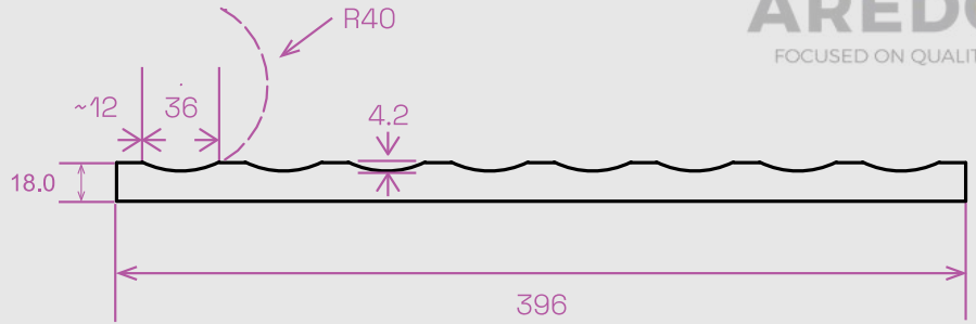
LAMEL KRAFT 4 detail
