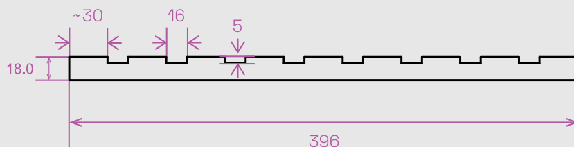
LAMEL PRIME 2 prierez
