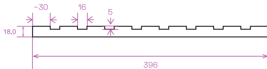
LAMEL PRIME 2 prierez
